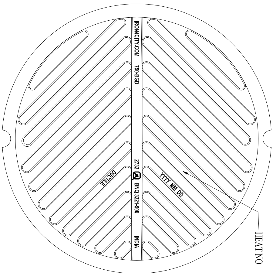
BHQ 3221-500/2017 DIMENSION
